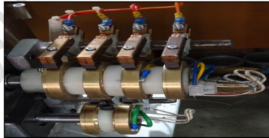
3. Slip Ring:
